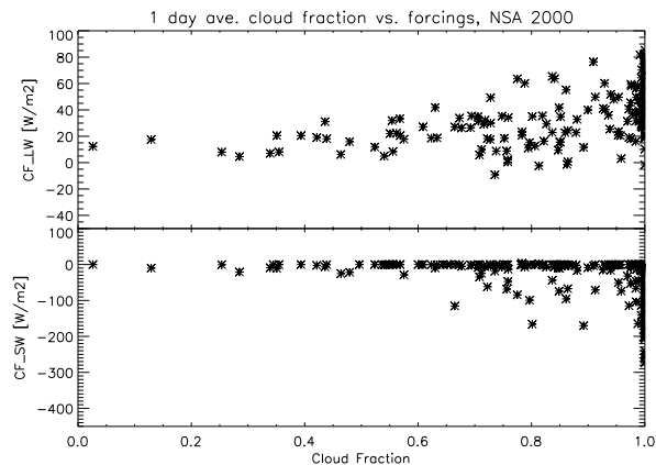
Fig. 4 . Scatterplot of CFLW (top) and CFSW (bottom) versus cloud fraction amount for NSA, 2002.
