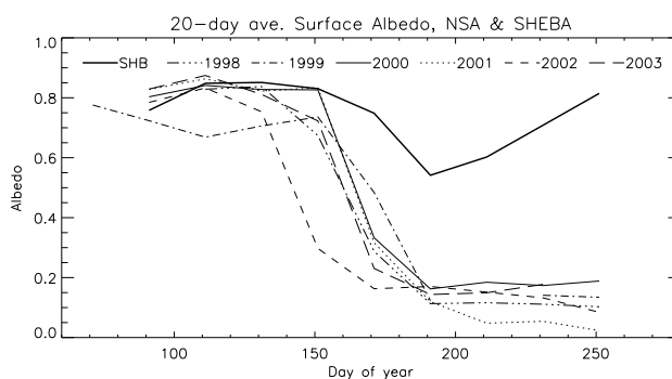
Fig. 3. Annual cycles of albedo for SHEBA (solid line) and six years of data from NSA.
