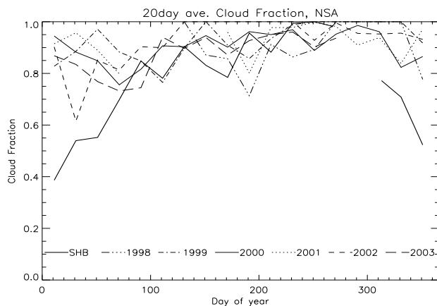
Fig. 2. 20-day averages of cloud fraction for SHEBA (solid line) and six years of data from NSA.
