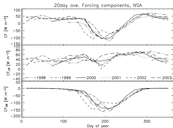
Fig. 1. Annual cycle of 20-day average a) Total, b) LW, and c) SW surface cloud forcing for SHEBA (bold line) plus six years of NSA data. All values in \text{Wm}^{-2} .
